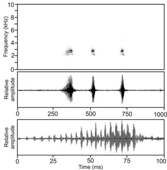
Fig. 9. Spectrogram, corresponding waveform, and expanded waveform (bottom) of the initial note of a regular note series emitted by Boophis boehmei . Recording obtained on 12 January 1992 at Andasibe (air temperature 23°C).
